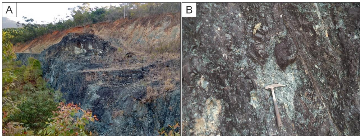
Figure 9: A) Landscape view of the Francisco IV quarry. B) Brecciated and highly foliated ultramafic rocks of the Quebra Osso Group.
