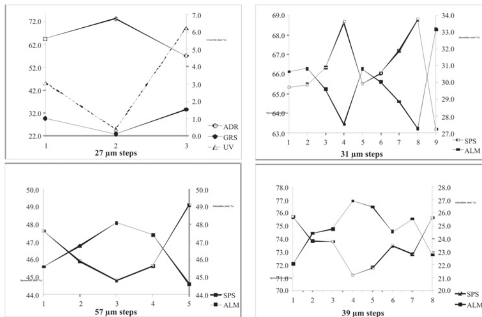
Figure 2 – Chemical zoning of single crystals of garnet (rim to rim) from the granitic rocks of Ciborro – Aldeia da Serra area, southern Portugal. a) Garnet from tonalite; b) garnet from pegmatite vein cutting coarse-grained biotite>muscovite granite; c) garnet from aplite-pegmatite vein cutting tonalite; d) garnet from pegmatite vein cutting mixed biotite granodiorite and granite. a) and b) Normal zoning; c) and d) reverse zoning.
