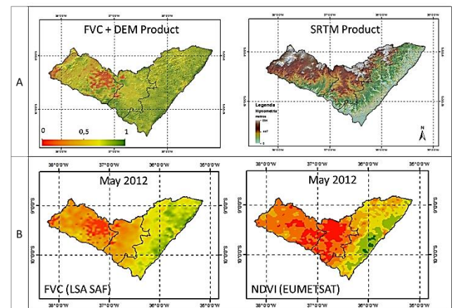
Figure 12. FVC, NDVI, DEM and SRTM products ingested into ILWIS
