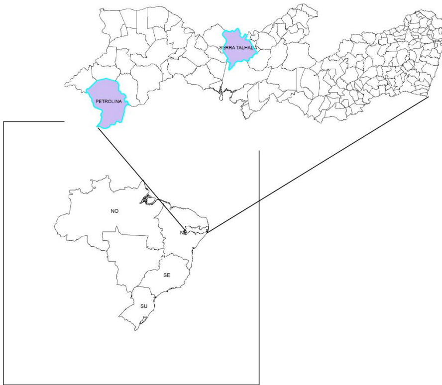
Figure 1. Spatial location of the municipalities Serra Talhada and Petrolina in Brazil.
