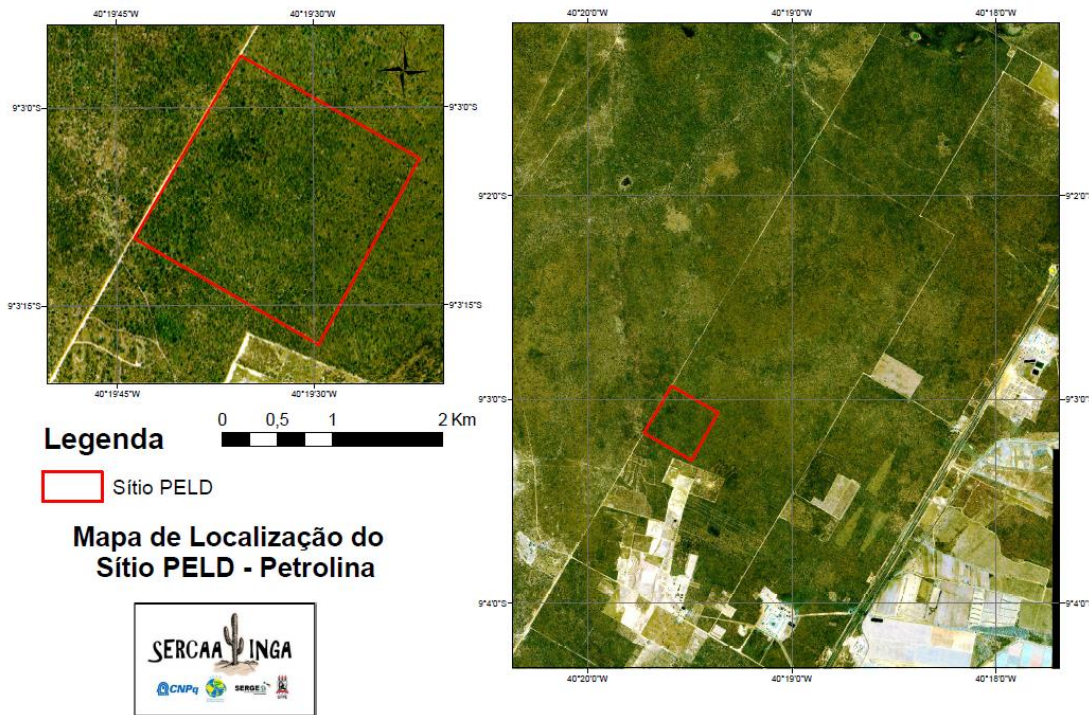
Figure 2. IKONOS Image, site 22, PELD, in Petrolina-PE.
