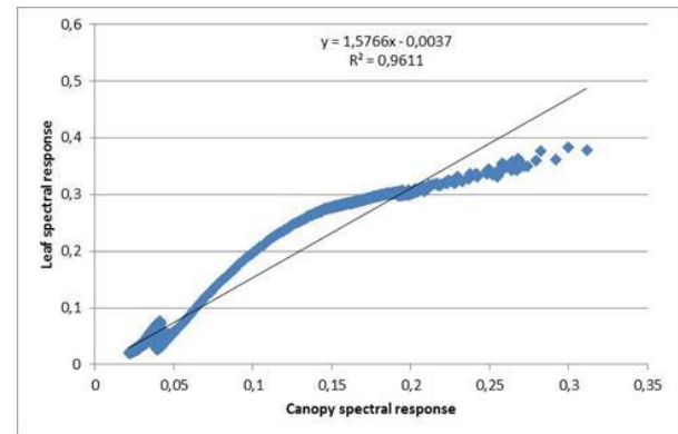
Figure 4. Relationship between canopy and leaf reflectance.
